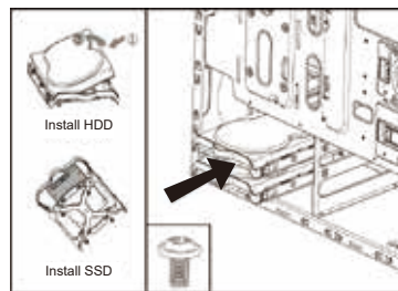
Insert the HDD into place
