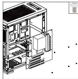
Install M/B
